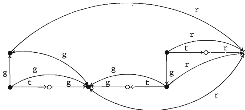
Figure 5: Illustration of the conditions of \text{can}\cdot\text{share} .
